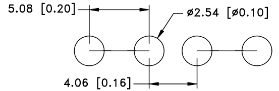
MOUNTING DETAIL
