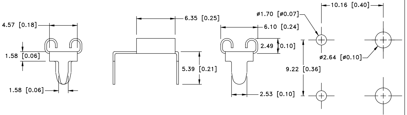
MOUNTING DETAIL FOR TWO CLIPS
