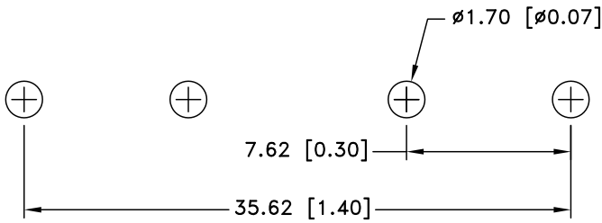
MOUNTING DETAIL
