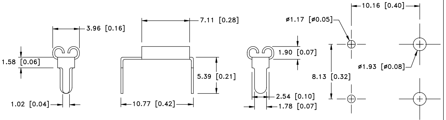
MOUNTING DETAIL FOR TWO CLIPS
