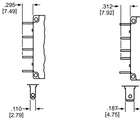
Auxiliary Switch
