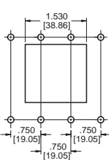
Mounting Detail*
