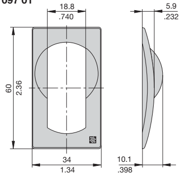
Snap-on frame with actuator guard (can be snapped on as switch-on protection or switch-off protection) Y 307 097 01
