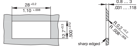
panel cut-out
