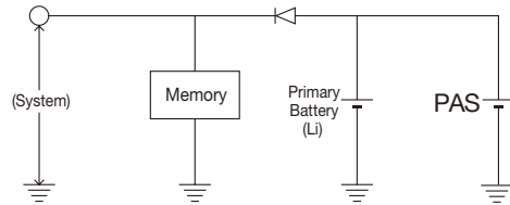
○Application 5: IC Memory card
