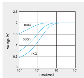
○充電特性(定抵抗) Charging characteristics (Constant R)
