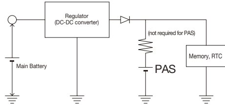
○Application 1: Cellular Phone
