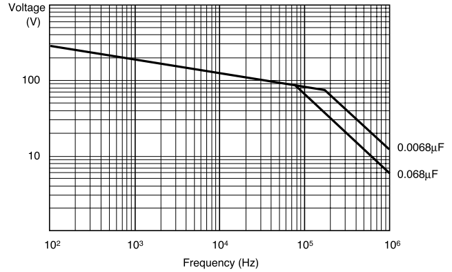
Rated 630VDC
