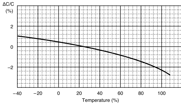
Capacitance change
