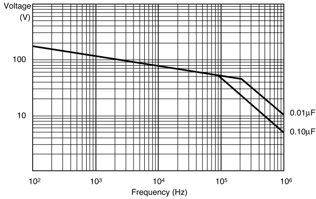
Rated 400VDC
