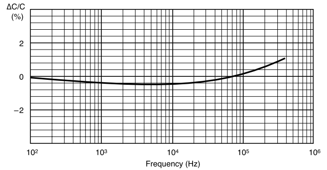
Capacitance change
