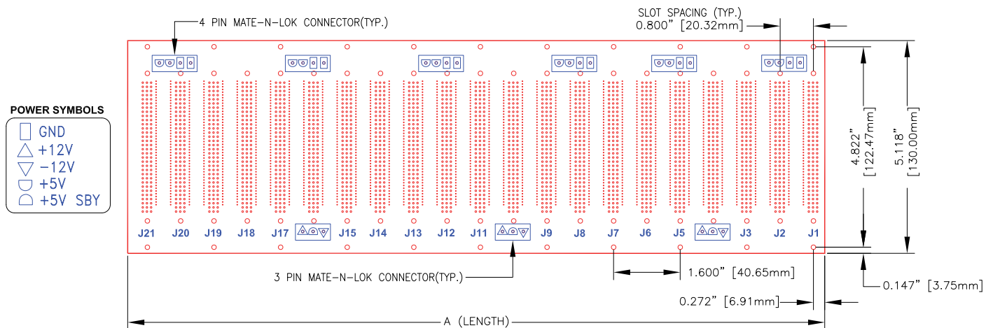
Power symbols indicate position and values of voltage and ground on a typical J1 VME backplane
