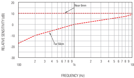
4x1.5 FREQUENCY RESPONSE
