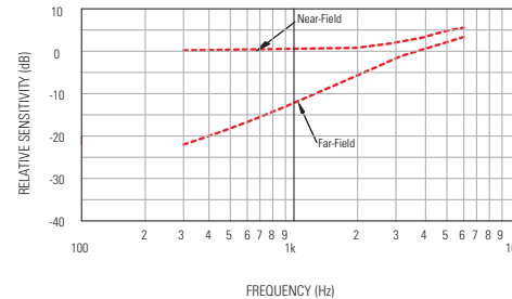
6x2.2 FREQUENCY RESPONSE
